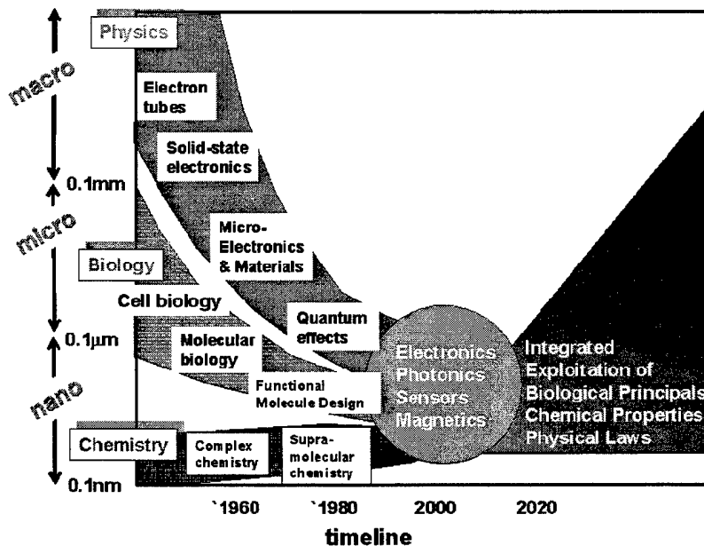
Figure 3-8. The time-evolution of the various physical sciences, plotted as a function of the length scale that represented the frontier of research in those fields.
